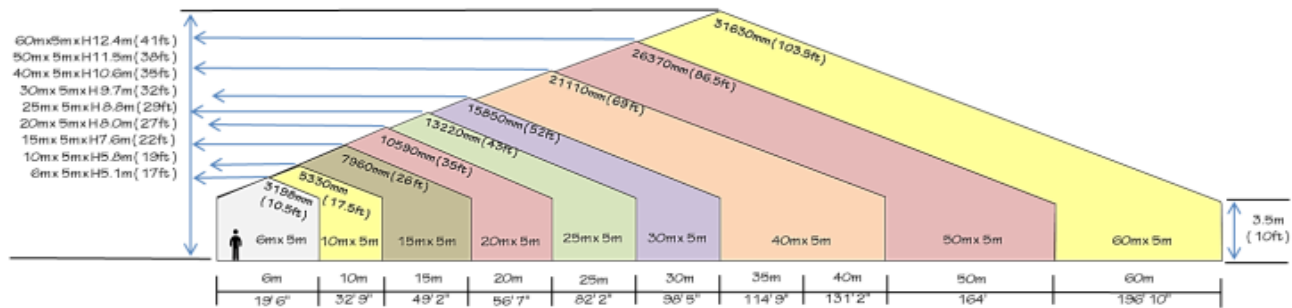
Marquee Tent 15m x 5m (2 block)
