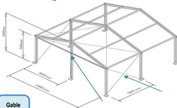
Gable Frame 15m
