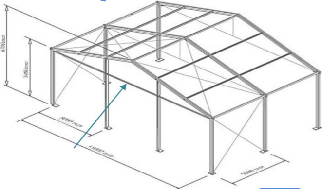
Marquee Safety Cross Rope
