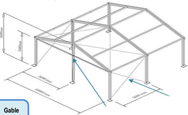
Marquee Tent 10m x 5m (2 block)
